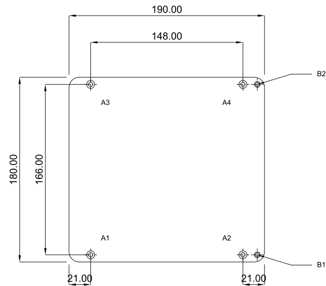
WALL MOUNTING HOLES COVER OPEN / FRONT VIEW
